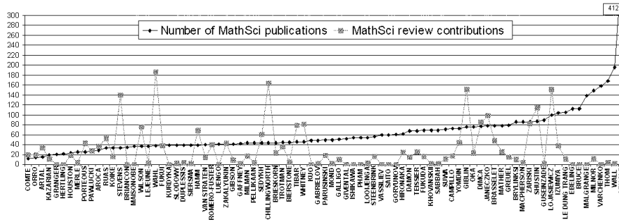
Figure 5. Publication counts for Singularity Theory authors compared to review contributions. Authors ranked by publication count (MathSci)
