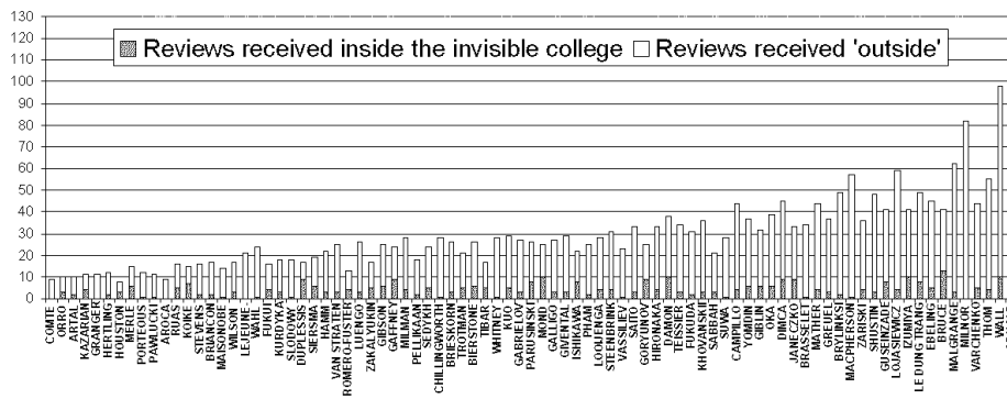
Figure 6. Reviews received by authors within Singularity Theory versus outside reviewers. Authors ranked by number of reviews received (MathSci)
